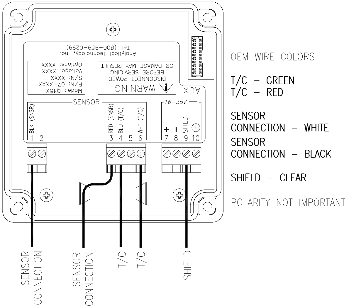
Figure 10 - OEM Sensor Connections
