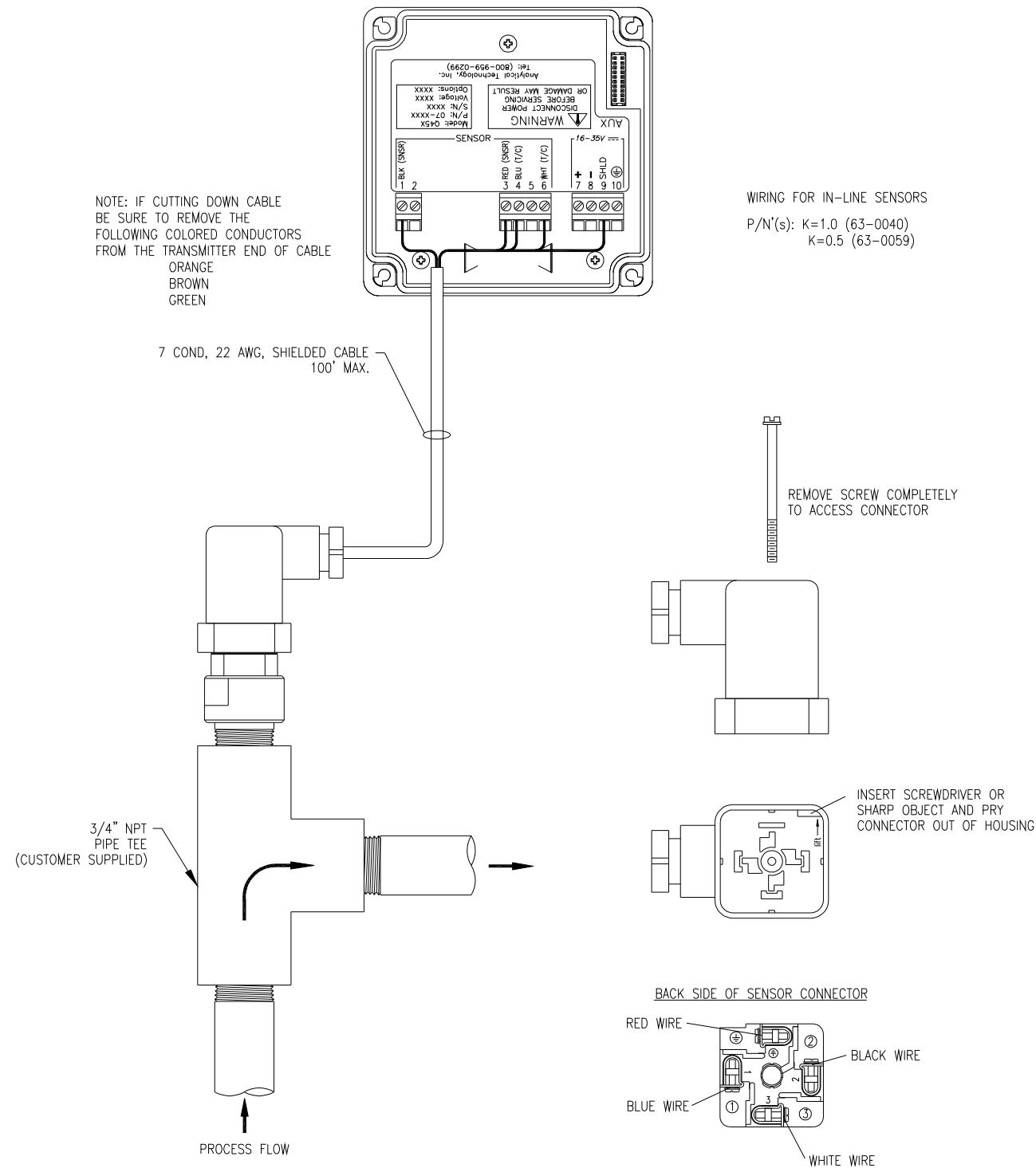
Figure 9 - In-Line Sensor Connection
