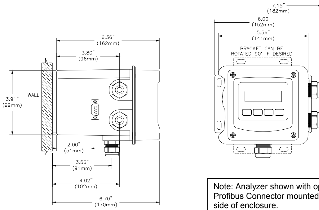
Figure 3 - Wall Mounting Dimensions
