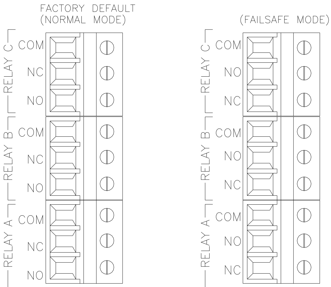
Figure 15 - Relay Connections
