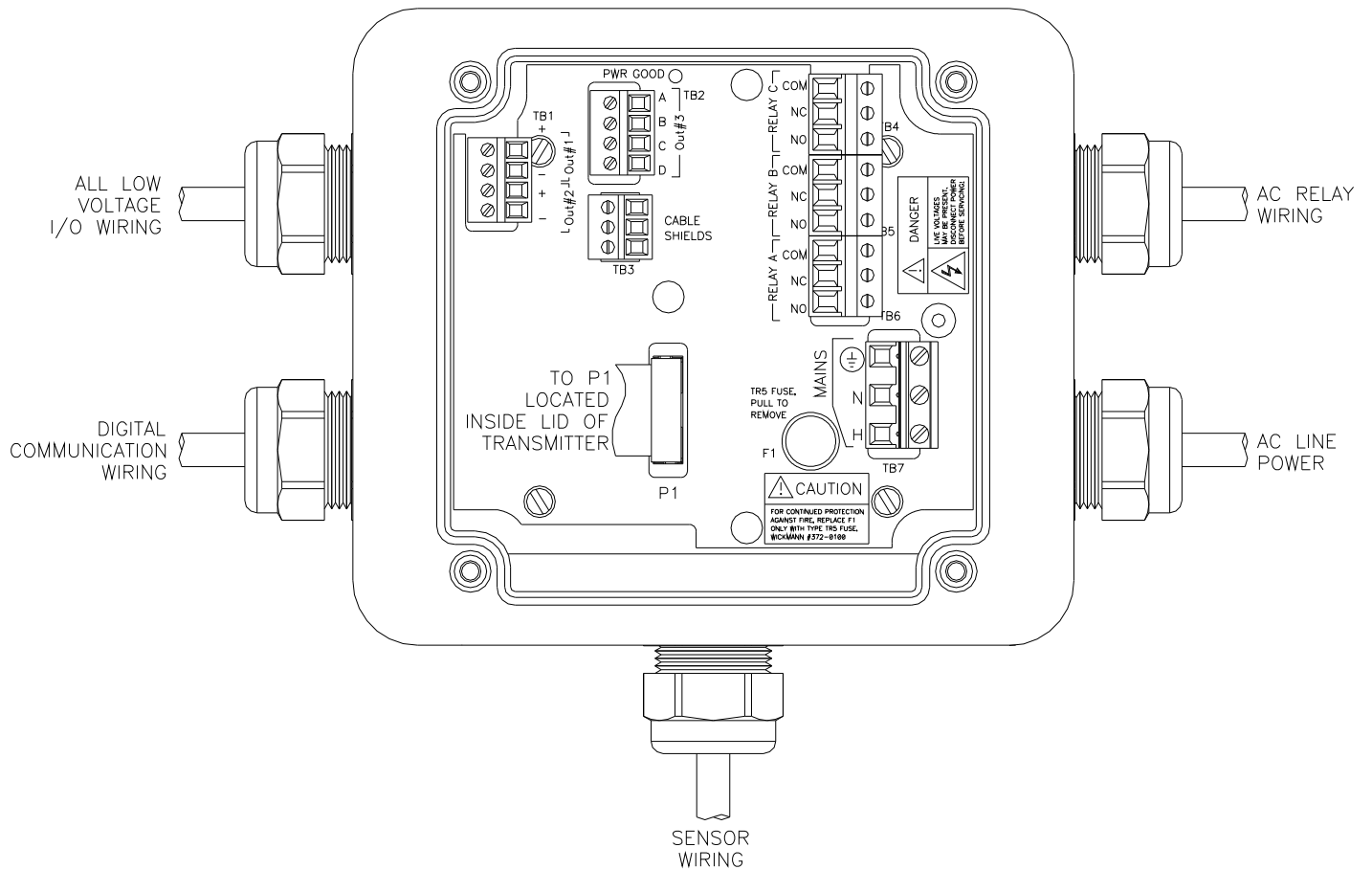
Figure 17 – Q46 Connections
