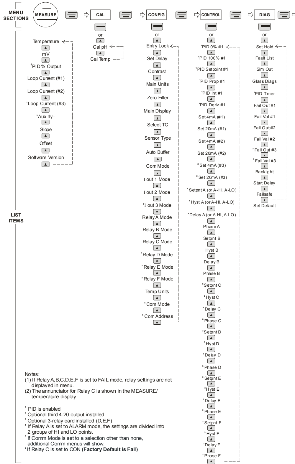
Figure 30 - Software Map
