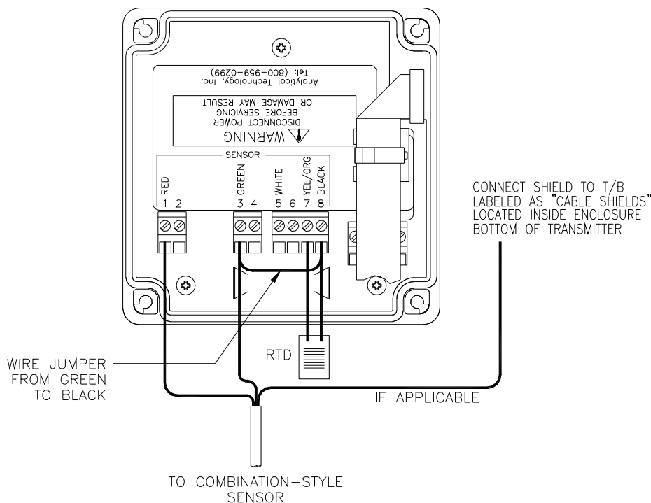
Figure 26 – OEM Sensor Connections, Combination Electrodes
