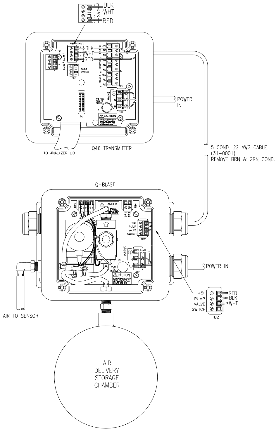
Figure 11 - Electrical Connections
