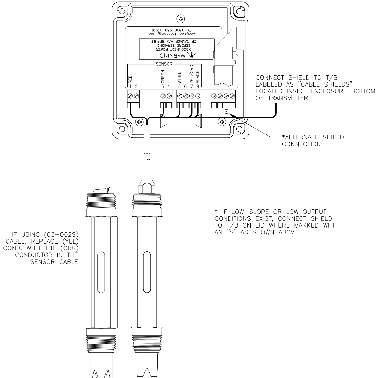
Figure 23 - Q46R Sensor Connections
