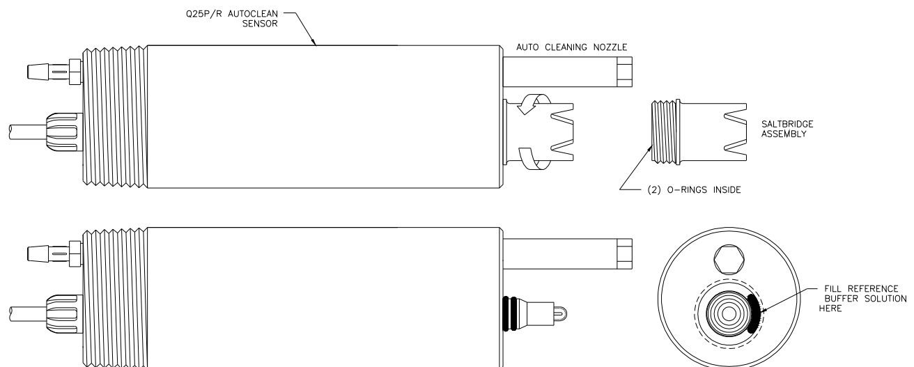
Figure 34 - Replacing the Saltbridge and Reference Buffer
