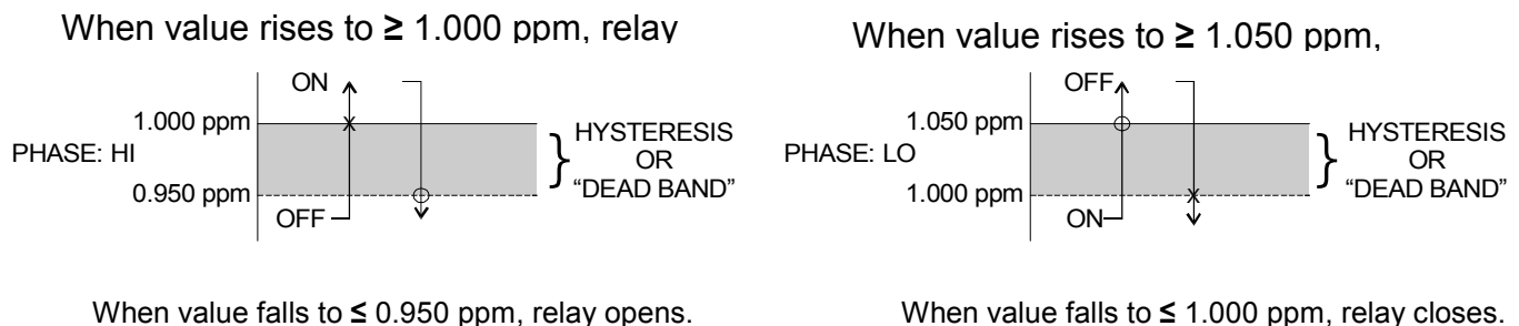
Figure 22 - Control Relay Example, Hysteresis & Phase Options
