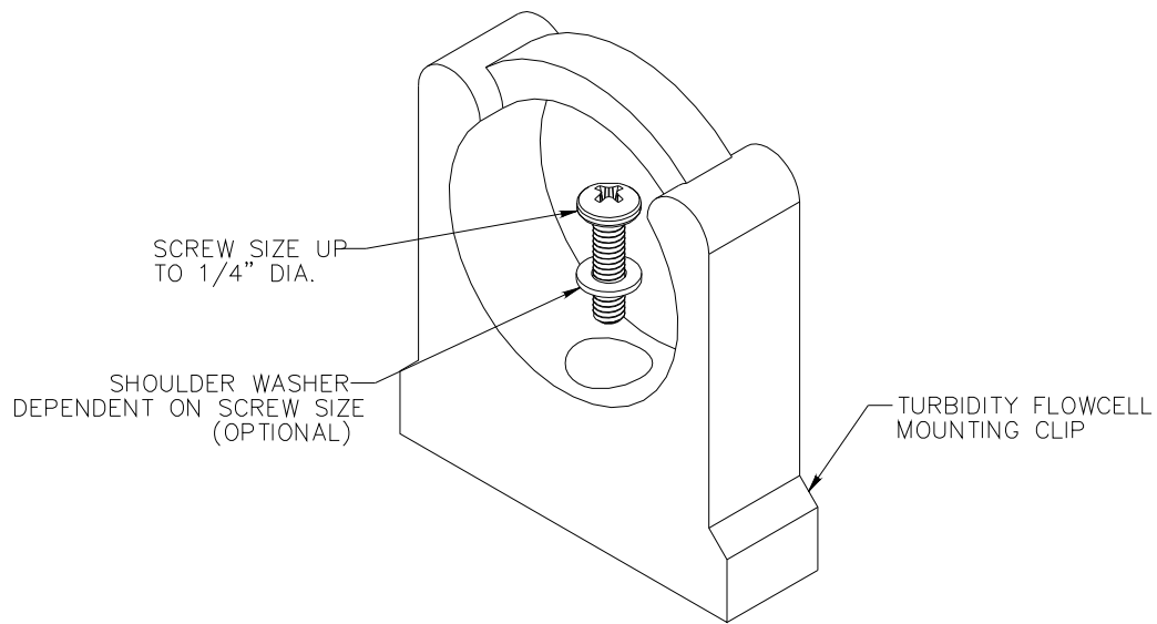
Figure 7 - Flowcell Clamp Diagram
