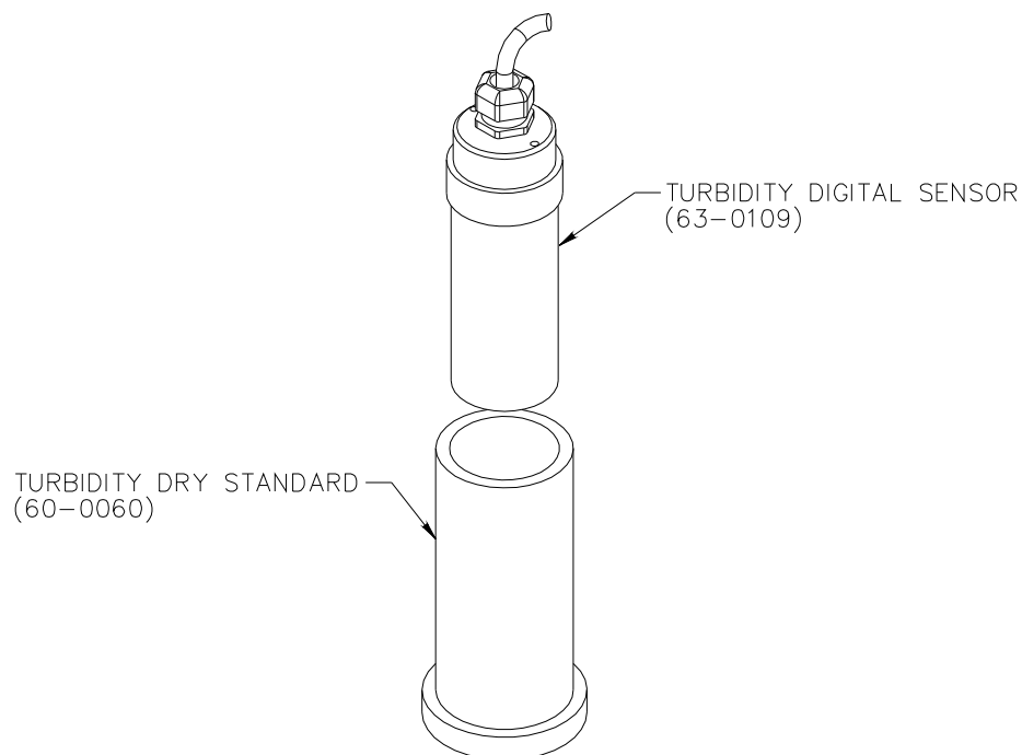
Figure 24 - Dry Standard Diagram
