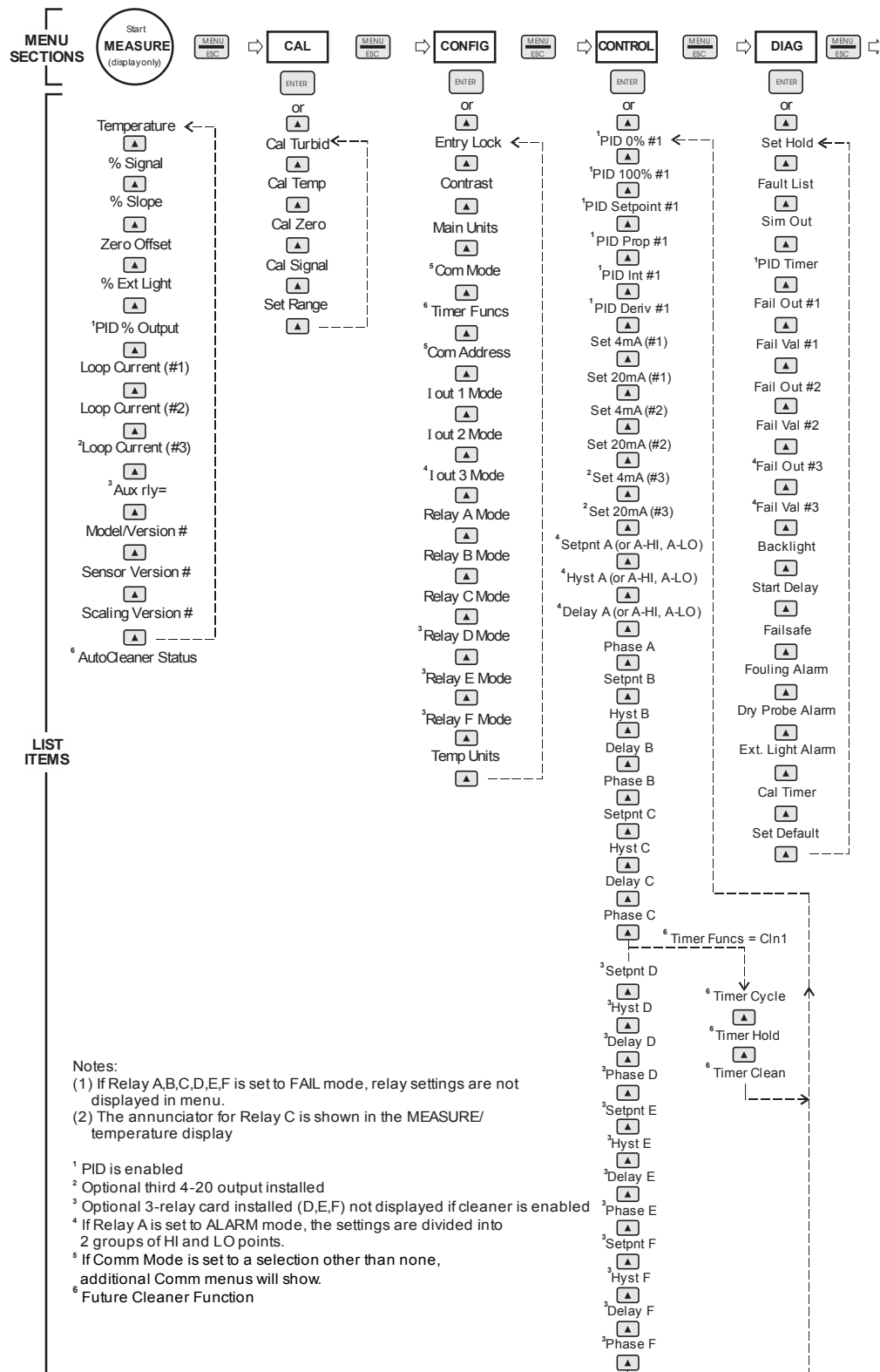
Figure 21 - Software Map
