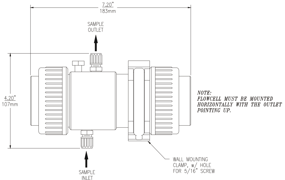
Figure 6 - Flowcell Dimensions
