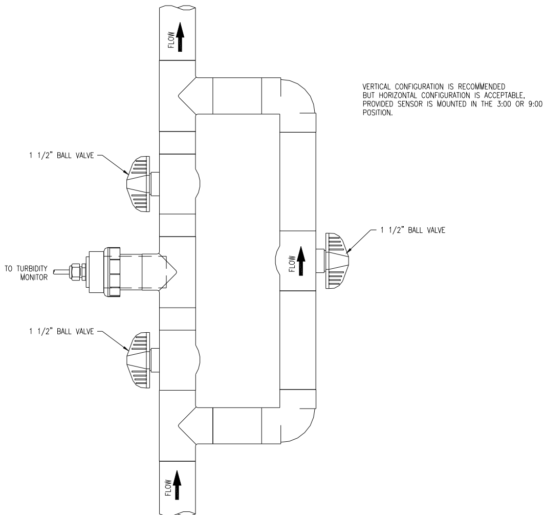
Figure 11 - 1 1/2" In-Line Installation
