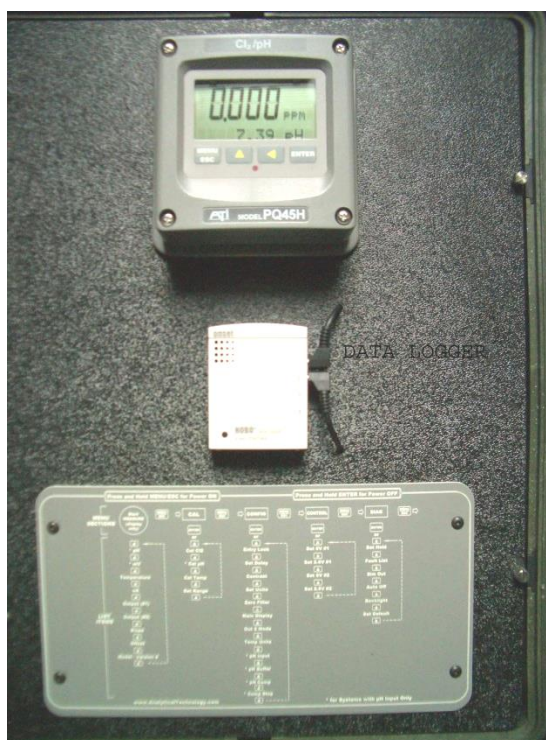
Figure 2 - Front View of Hinged Panel
